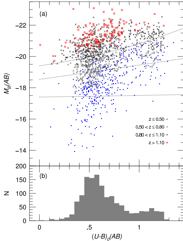
FIG. 18.— Rest-frame color-magnitude diagram and color distribution. (a) Rest-frame brightness vs. color for galaxies with TKRS redshifts in the Giavalisco et al. (2004) catalog. The three dashed lines show the limiting absolute magnitude as a function of rest-frame color at three different redshifts: z = 0.50 (lower curve), z = 0.80 (middle curve) and z = 1.10 (top curve). The symbols are also coded by redshift interval as shown in the figure. (b) Distribution of (U - B)_0 colors in 0.05 mag bins. The trough at (U - B)_0(AB) \approx 0.9 is consistent with that seen in other samples of galaxies.
